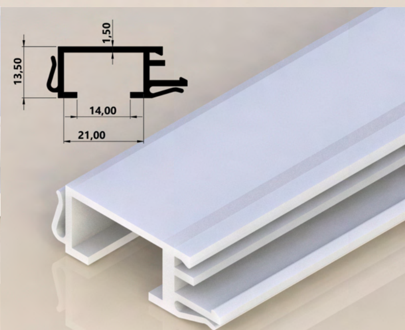
PERFIL RIGIDO 21,00X13,50X1,50MM
